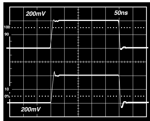
Figure 28. Noninverting Small Signal Pulse Response, R_L = 1 k \Omega
