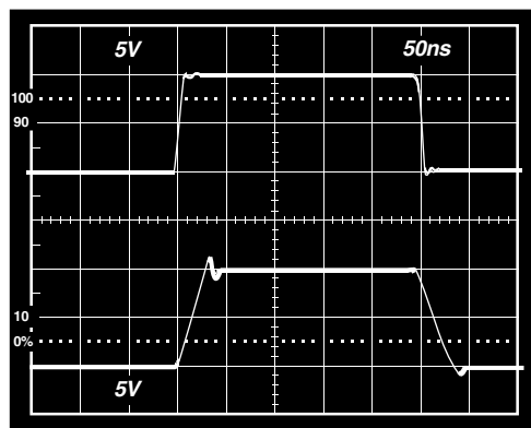
Figure 26. Noninverting Large Signal Pulse Response, R_L = 1 k \Omega
