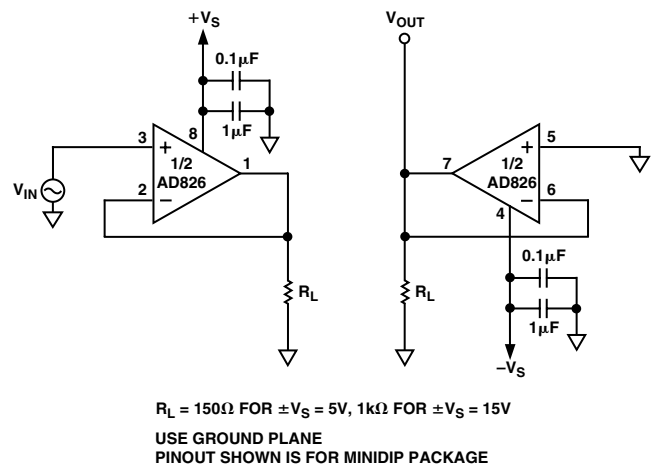
Figure 24. Crosstalk Test Circuit
