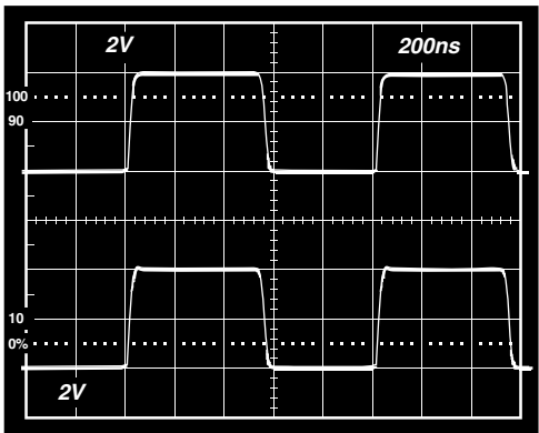
Figure 39. Pulse Response
